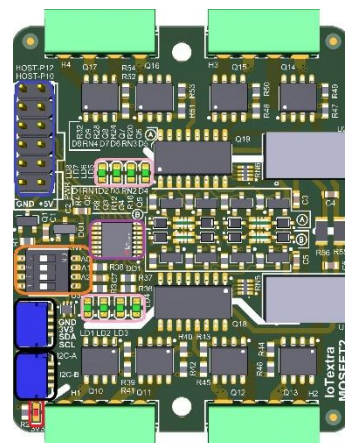
HOST-P12 and Qwiic®
